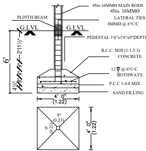
FOUNDATION DETAIL (SCALE: 1:50)
