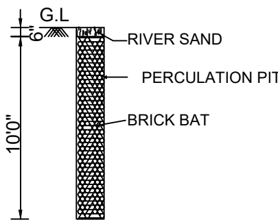
PERCULATION PIT
