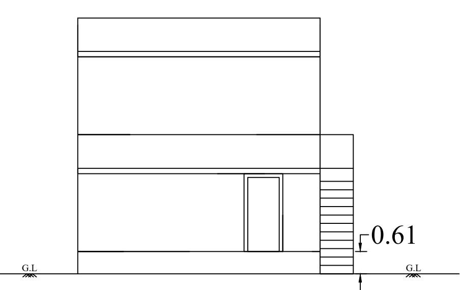
FRONT ELEVATION
