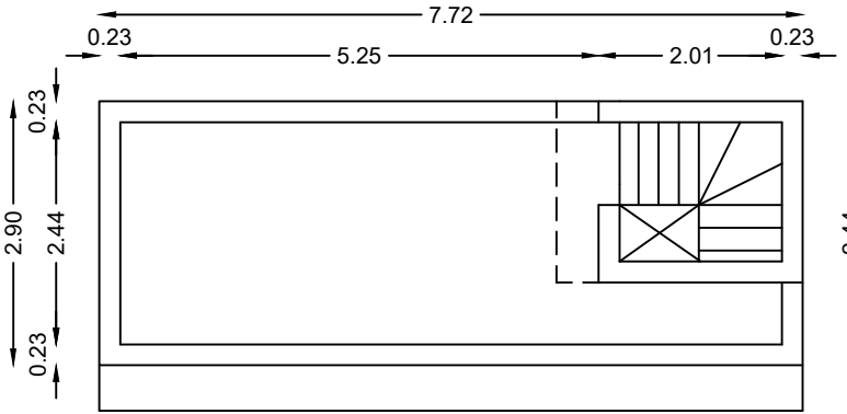
OPEN TERRACE
