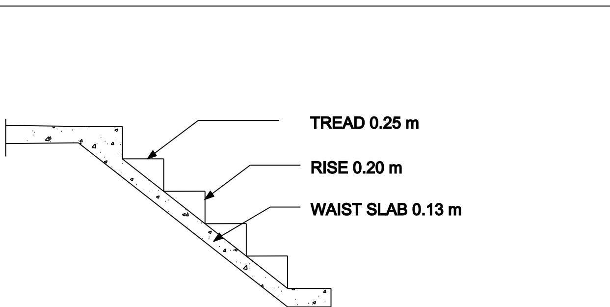
STAIR DETAILS
