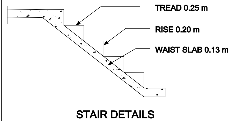
STAIR DETAILS
