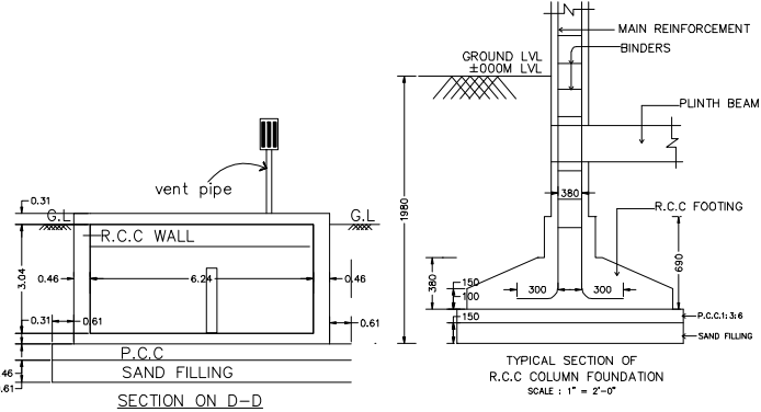
SECTION ON D-D
