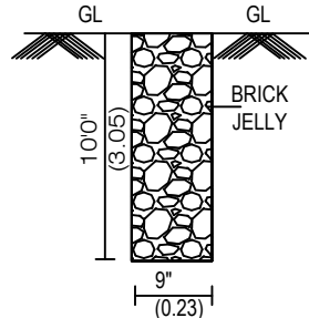
PERCOLATION PIT:-
