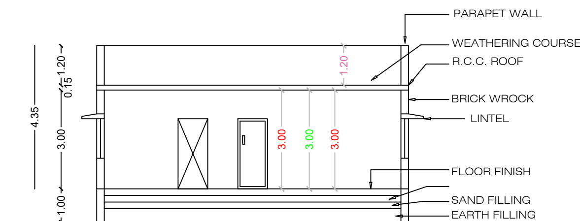
SECTION ON "XY"
