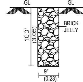
PERCULATION PIT:-
