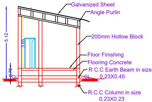
SECTION ON "PQ" SCALE 1:100
