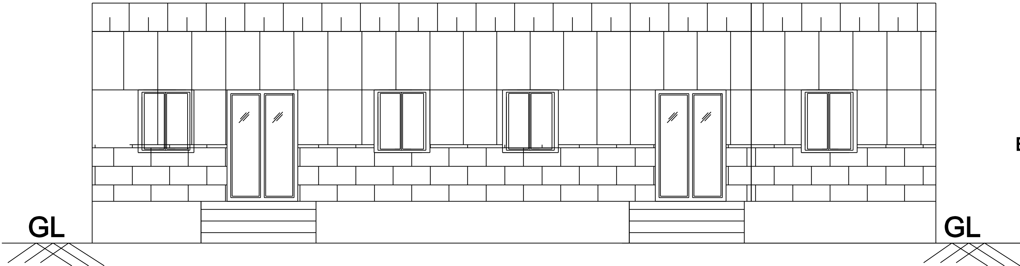
FRONT ELEVATION
