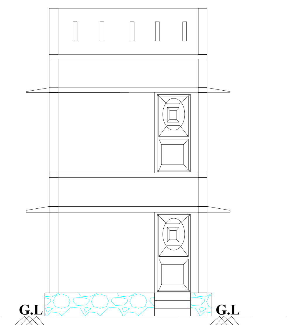
FRONT ELEVATION
