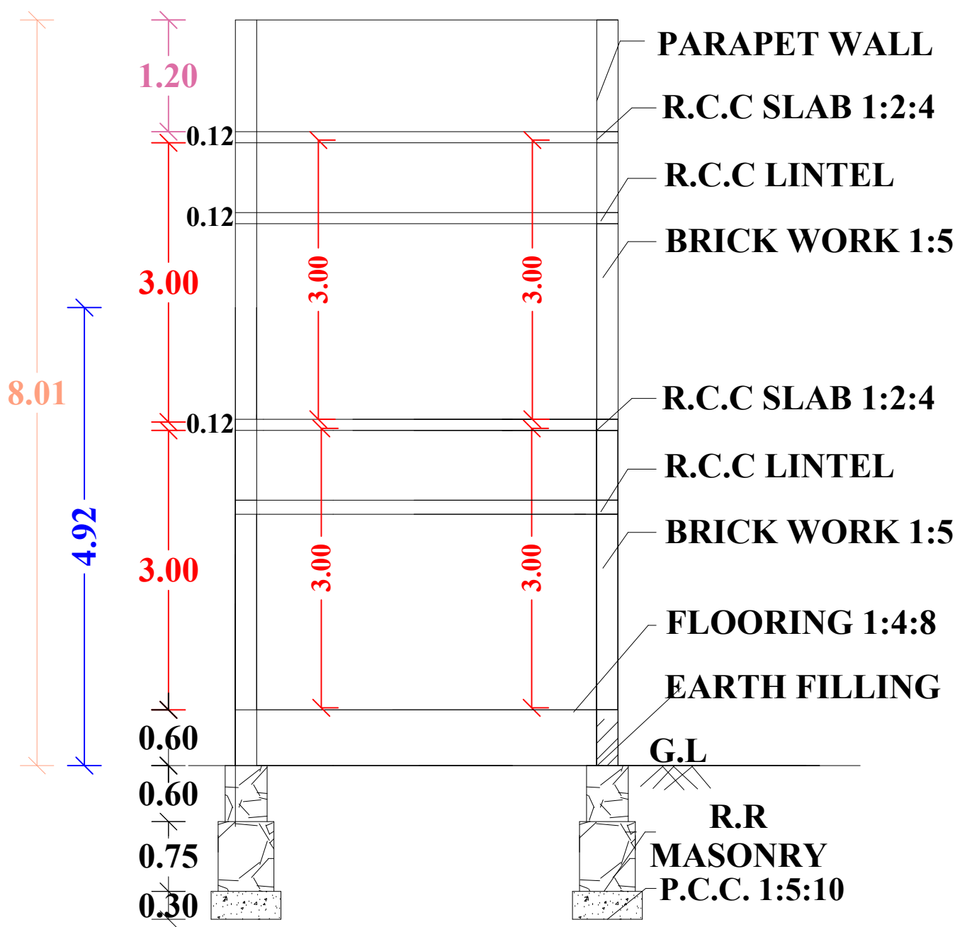
"SECTION "AB"
