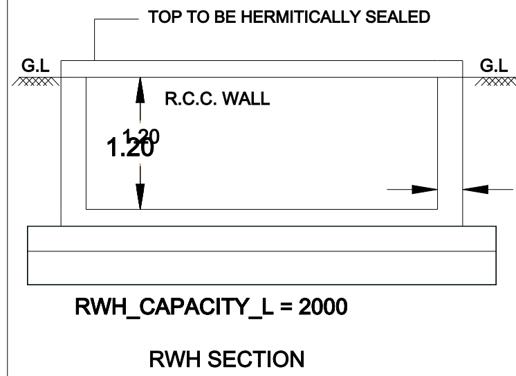
RW H SECTION
