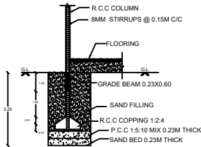
FOUNDATION DETAILS
