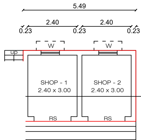
SED GROUND FLOOR PLAN
