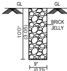
PERCULATION PIT:-
