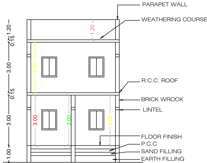
SECTION ON "XY"
