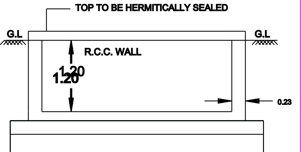
RWH_SECTION
