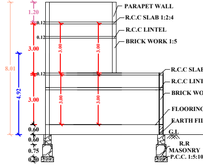
"SECTION 'AB'"
