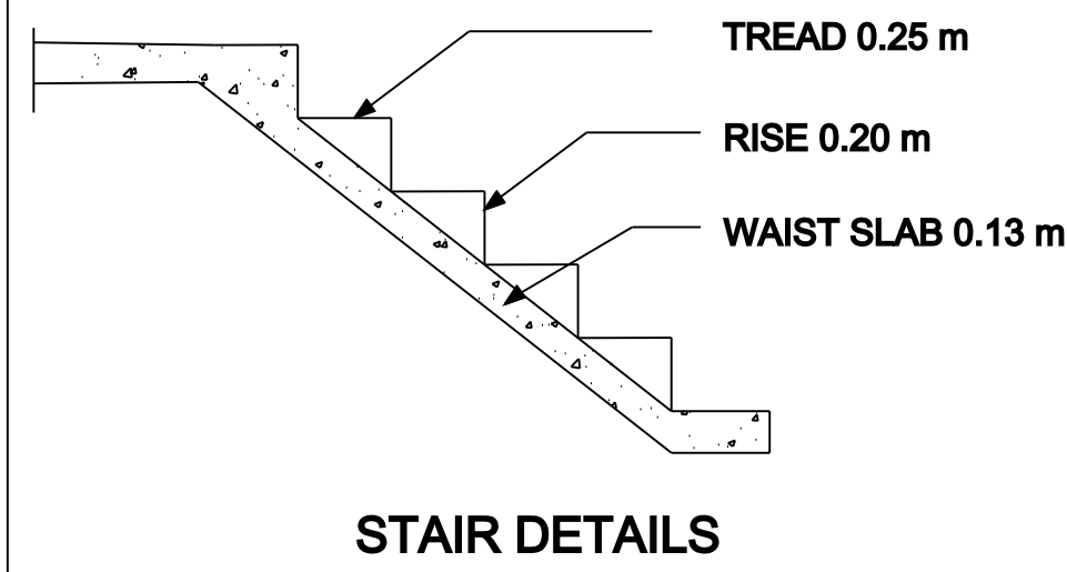
STAIR DETAILS
