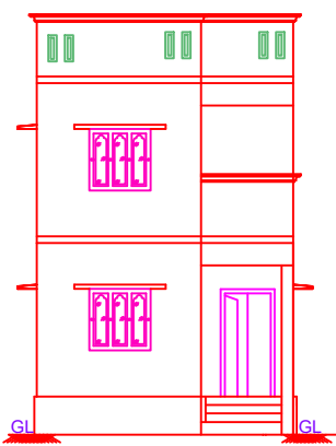
FRONT ELEVATION
