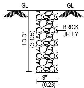
PERCOLATION PIT:-
