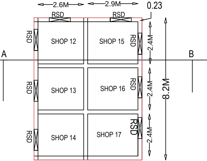
PROPOSED FIRST FLOOR PLAN,1:100
