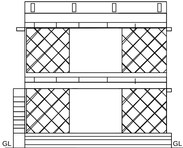
NORTH FACE ELEVATION
