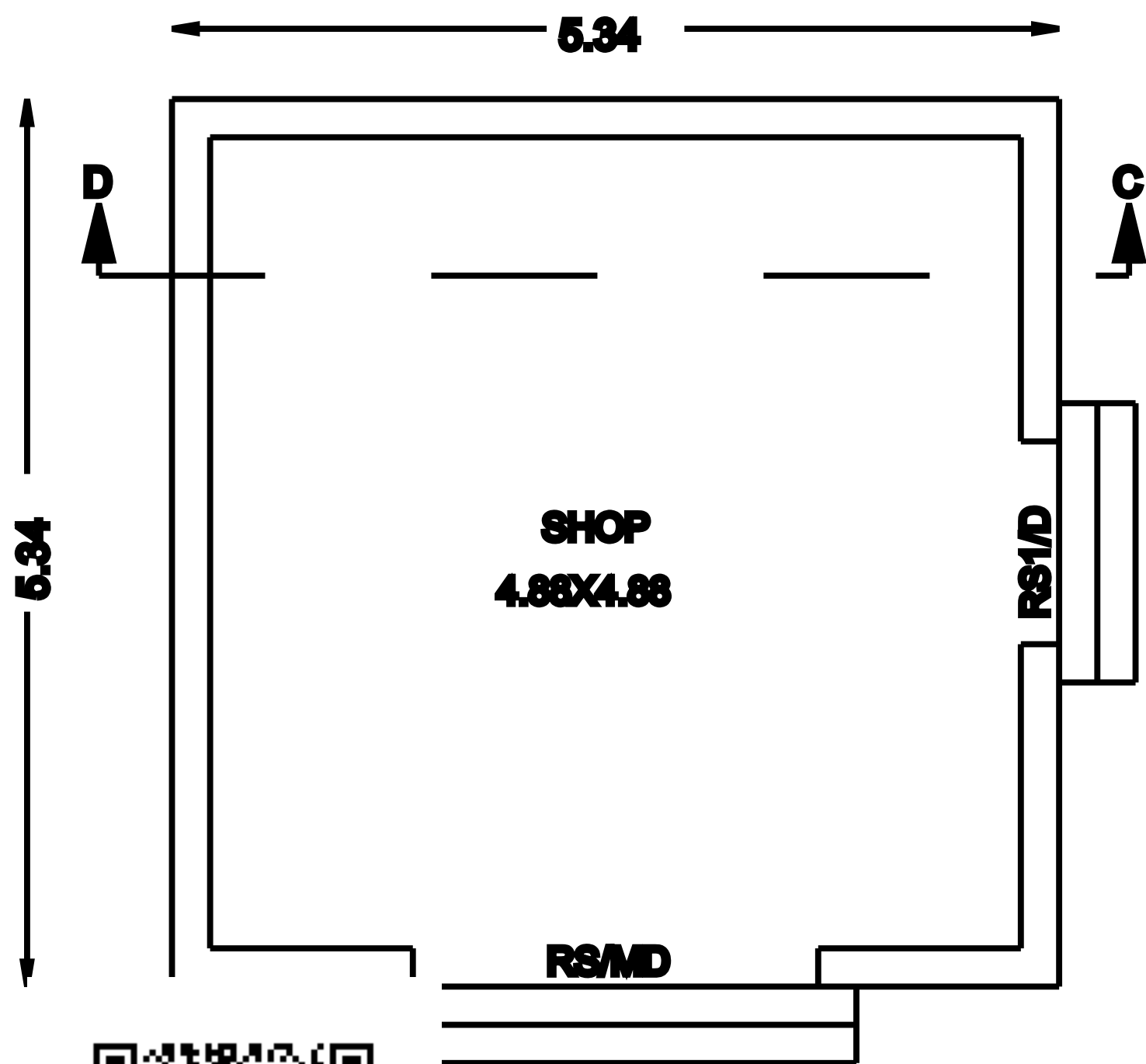
PLAN
