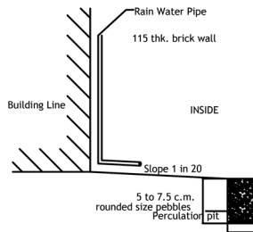
PERCOLATION PIT
