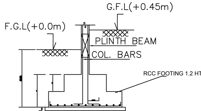
SECTION X-X OF FOOTING SCALE - 1:75
