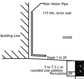
PERCOLATION PIT
