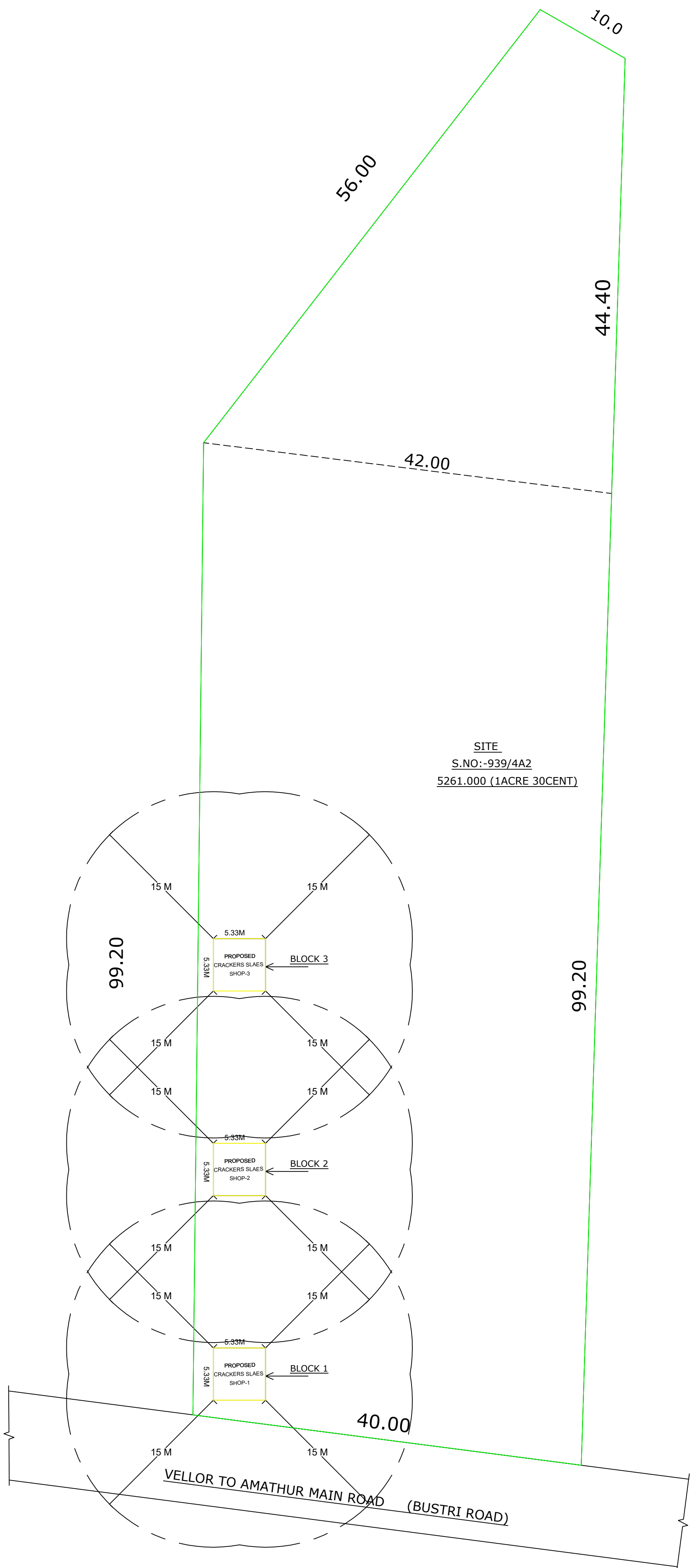
SITE PLAN SCALE 1CM:3M
