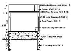
SECTION ON AB
