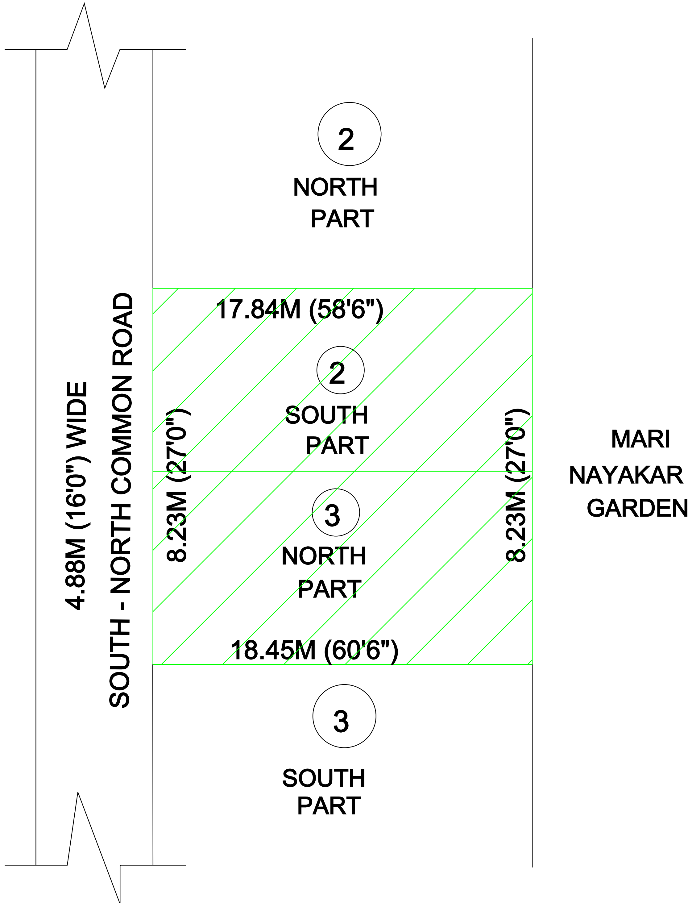
LOCATION PLAN
