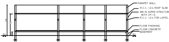
SECTION ON AA'
