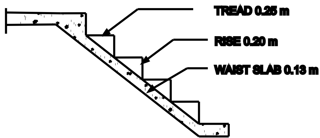
STAIR DETAILS
