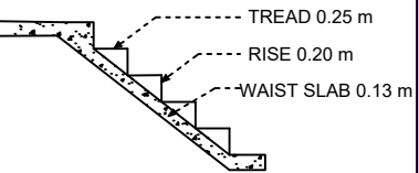
STAIR DETAILS
