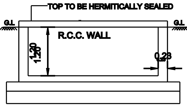
RWH SECTION ( SAMPLE ) RWH_CAPACITY_L=2000
