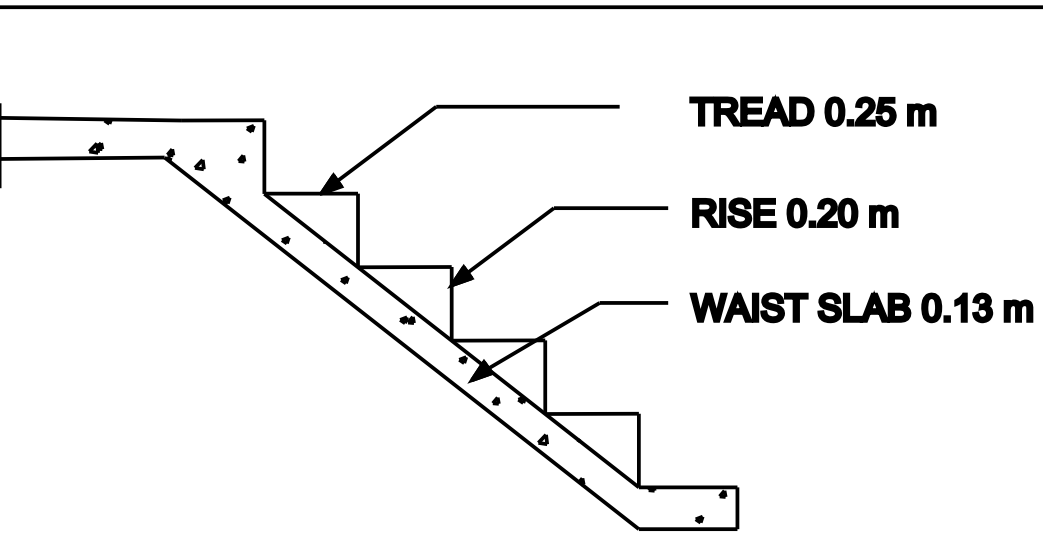
STAIR DETAILS
