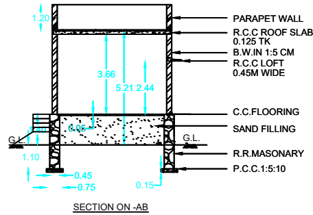
SECTION ON-AB
