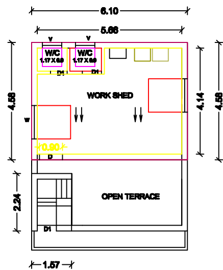
PROPOSED TIN SHEET ROOF COMMERCIAL BUILDING IN FIRST FLOOR PLAN
