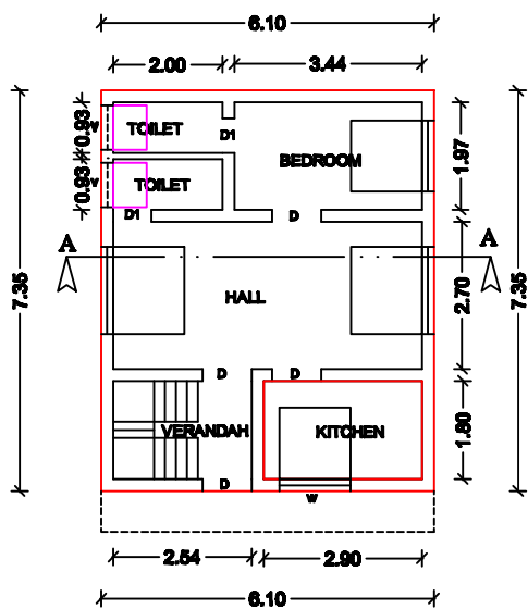
EXISTING RCC ROOF RESIDENTIAL BUILDING IN GROUND FLOOR PLAN
