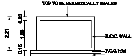
SECTION ON "U.G.SUMP"
