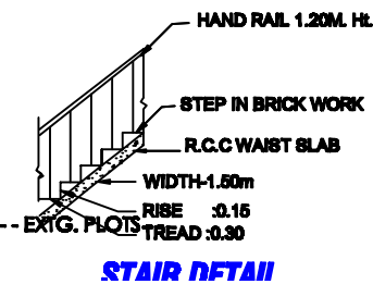
STAIR DETAIL
