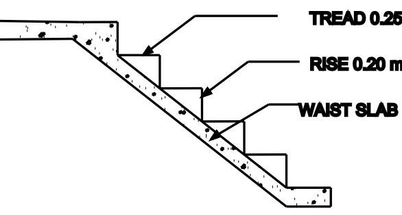
STAIR DETAILS
