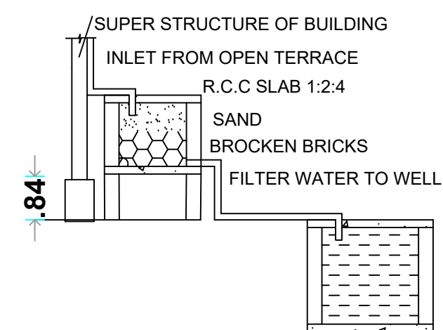
RAINWATER HARVESTING
