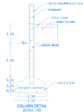
COLUMN DETAIL (SCALE 1:50)
