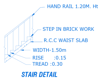
STAIR DETAIL
