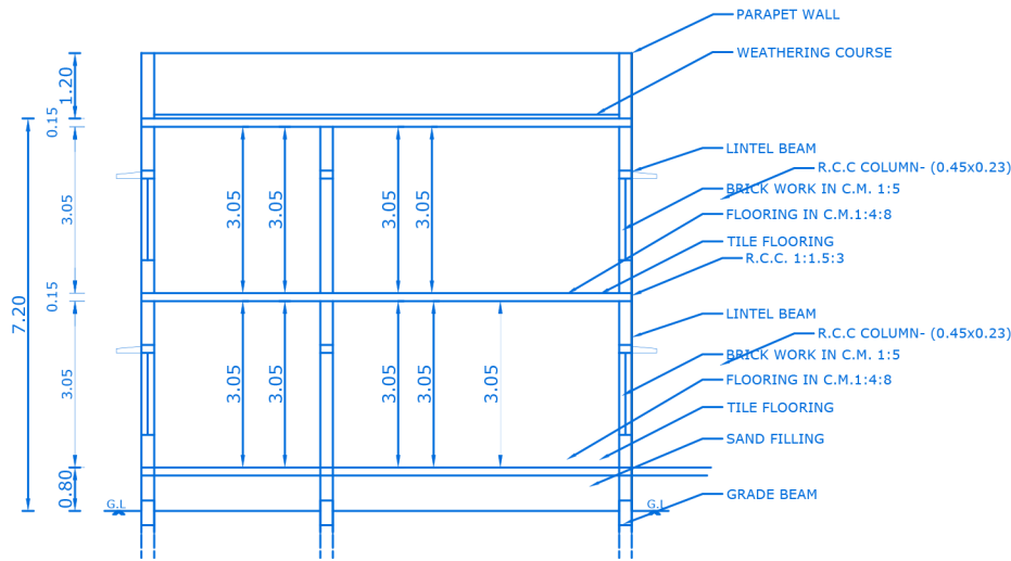
SECTION ON AA SECTION ON AA
