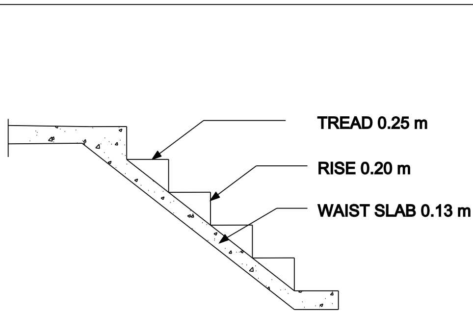
STAIR DETAILS
