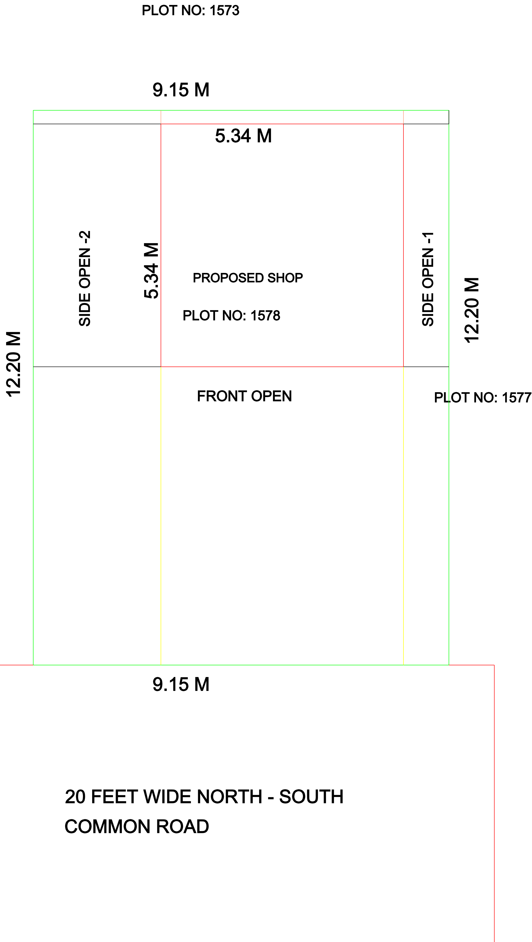
SITE PLAN
