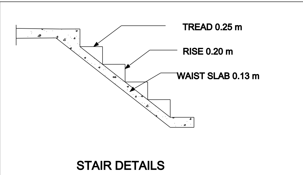
STAIR DETAILS
