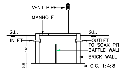
SECTION OF SEPT. TANK
