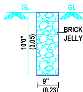
PERCULATION PIT
