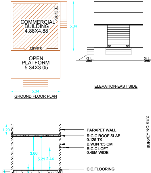
BUILDING PLAN SCALE 1:100
