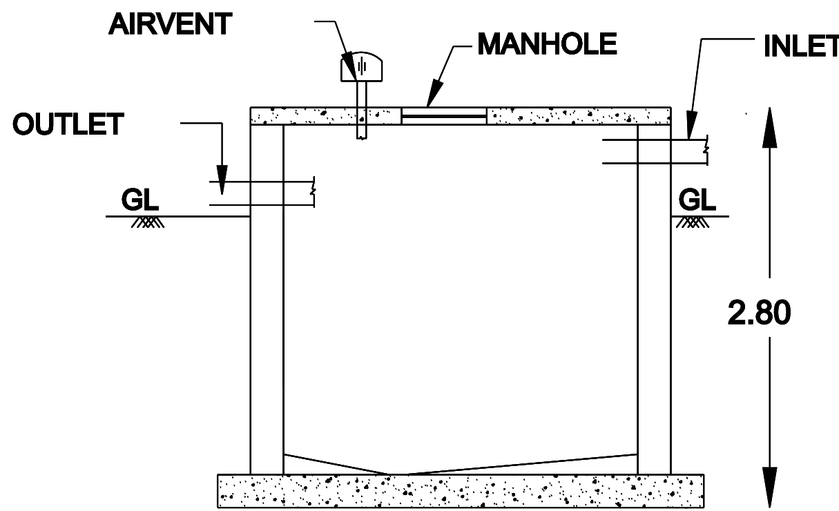
SECTION B-B' PLAN SEPTIC TANK
