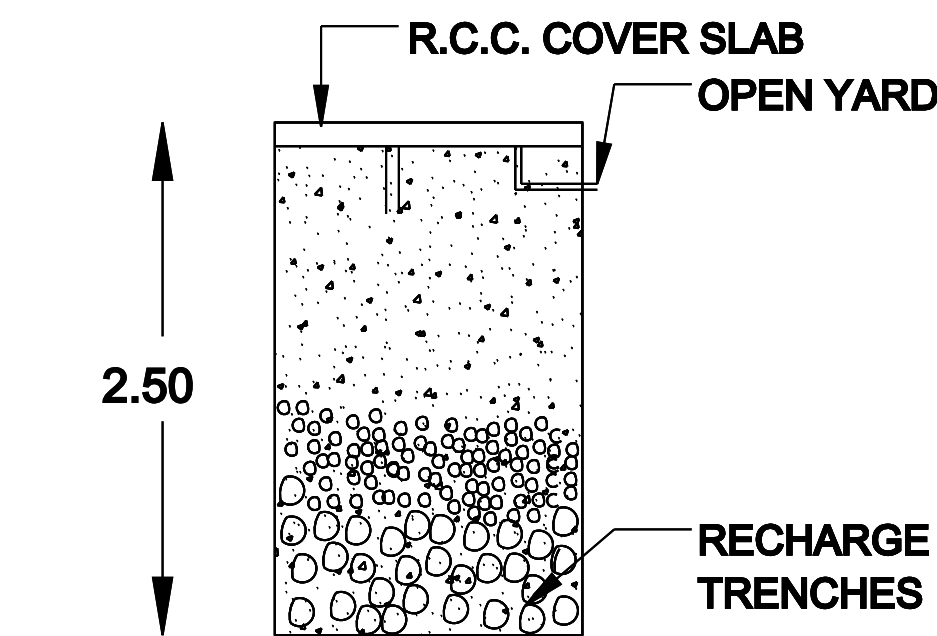
SECTION C-C' RWHT_CAPACITY_L=2000LTRS PLAN R.W.H
