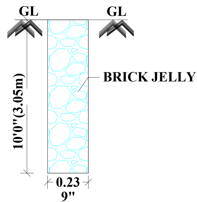
PERCOLATION PIT
