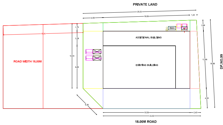
SITE PLAN
