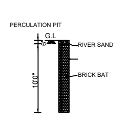
PERCULATION PIT
