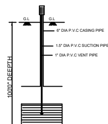
BORE WELL
