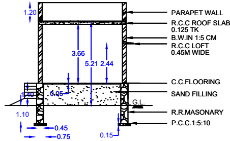
SECTION ON-AB
