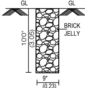
PERCULATION PIT:-
