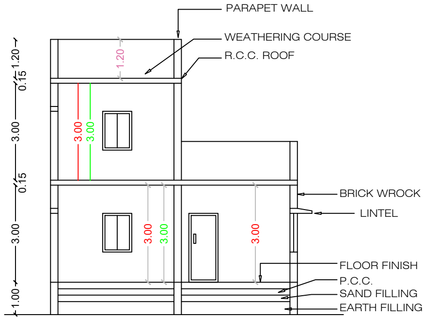
SECTION ON "XY"
