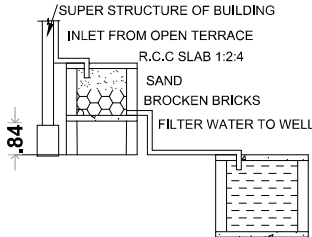
RAINWATER HARVESTING
