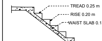
STAIR DETAILS
