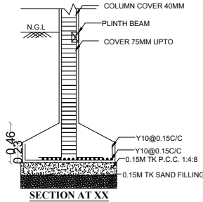
SECTION AT XX
