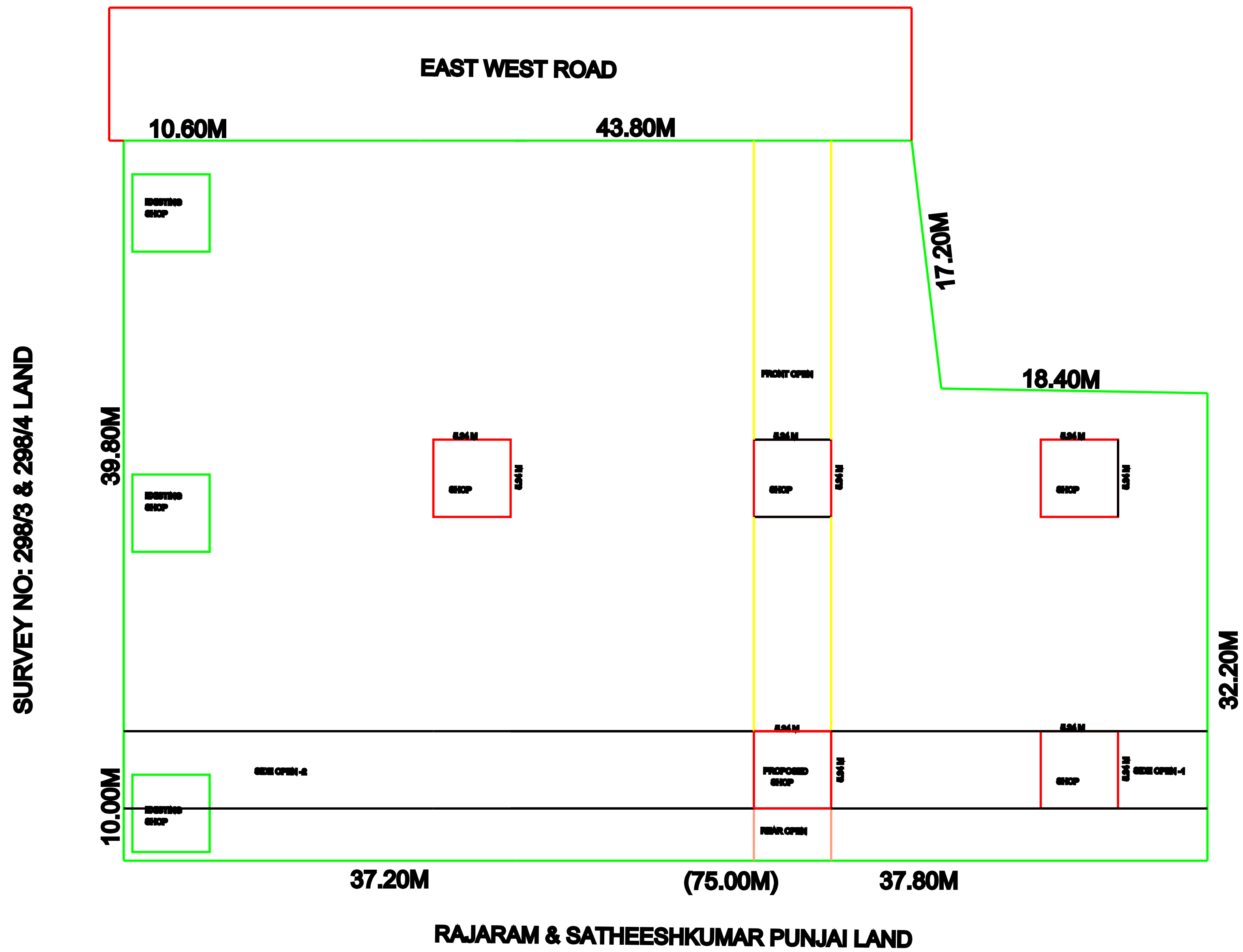
SITE PLAN
